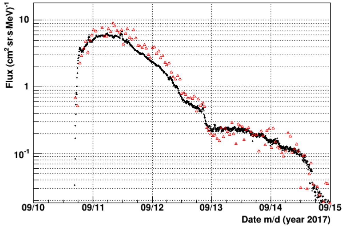
45.0 MeV H PROBA-V/EPT (red) and GOES-13 (black) flux
