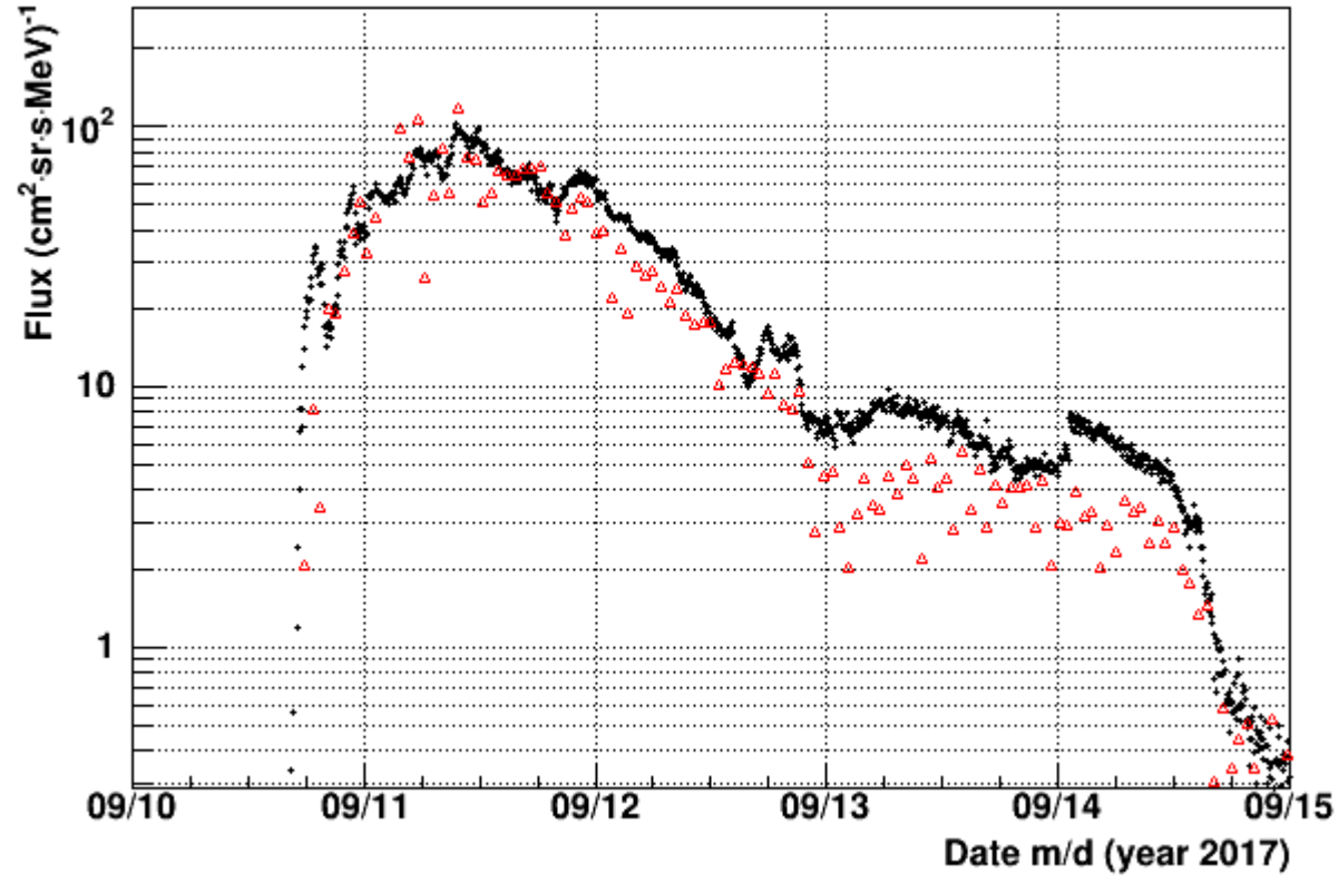
11.2 MeV H PROBA-V/EPT (red) and GOES-13 (black) flux
