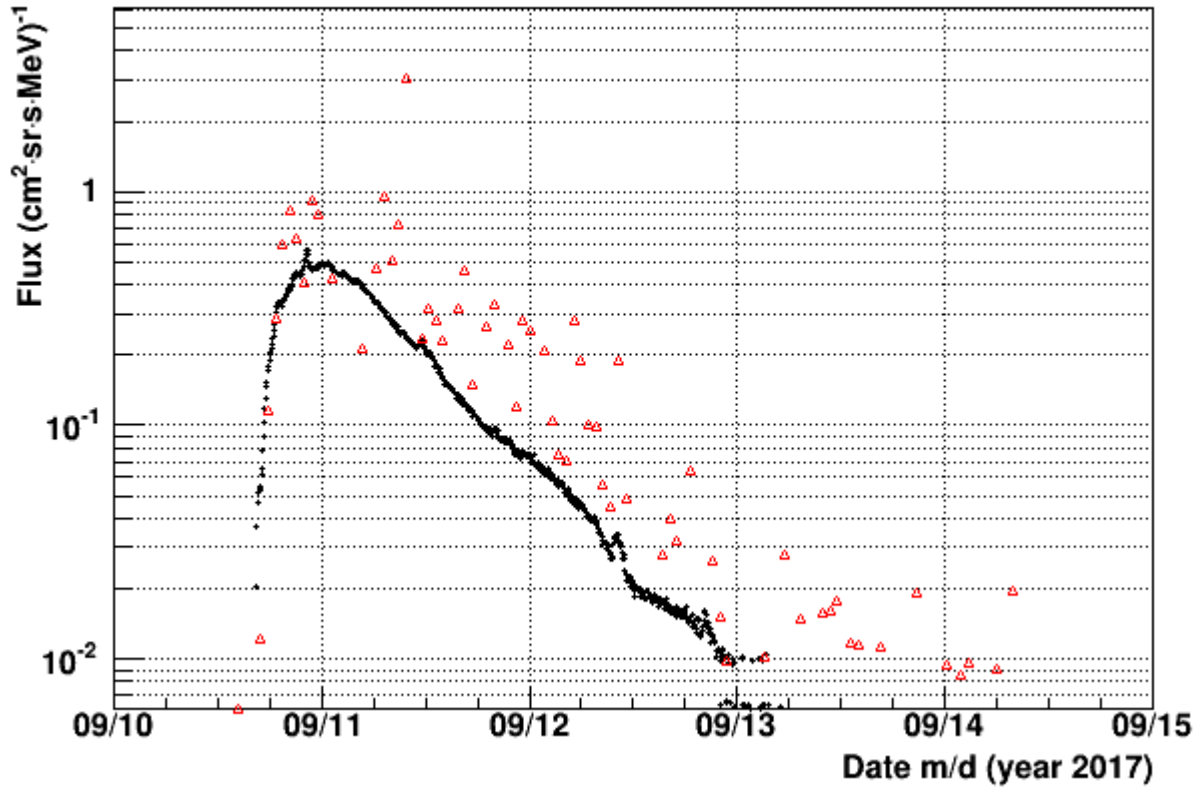
109 MeV H PROBA-V/EPT (red) and GOES-13 (black) flux
